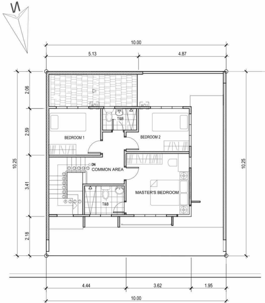
BLOCK 3, LOT 10-UNIT 2B 2 SECOND FLOOR PLAN SCALE 1:100 MTS
