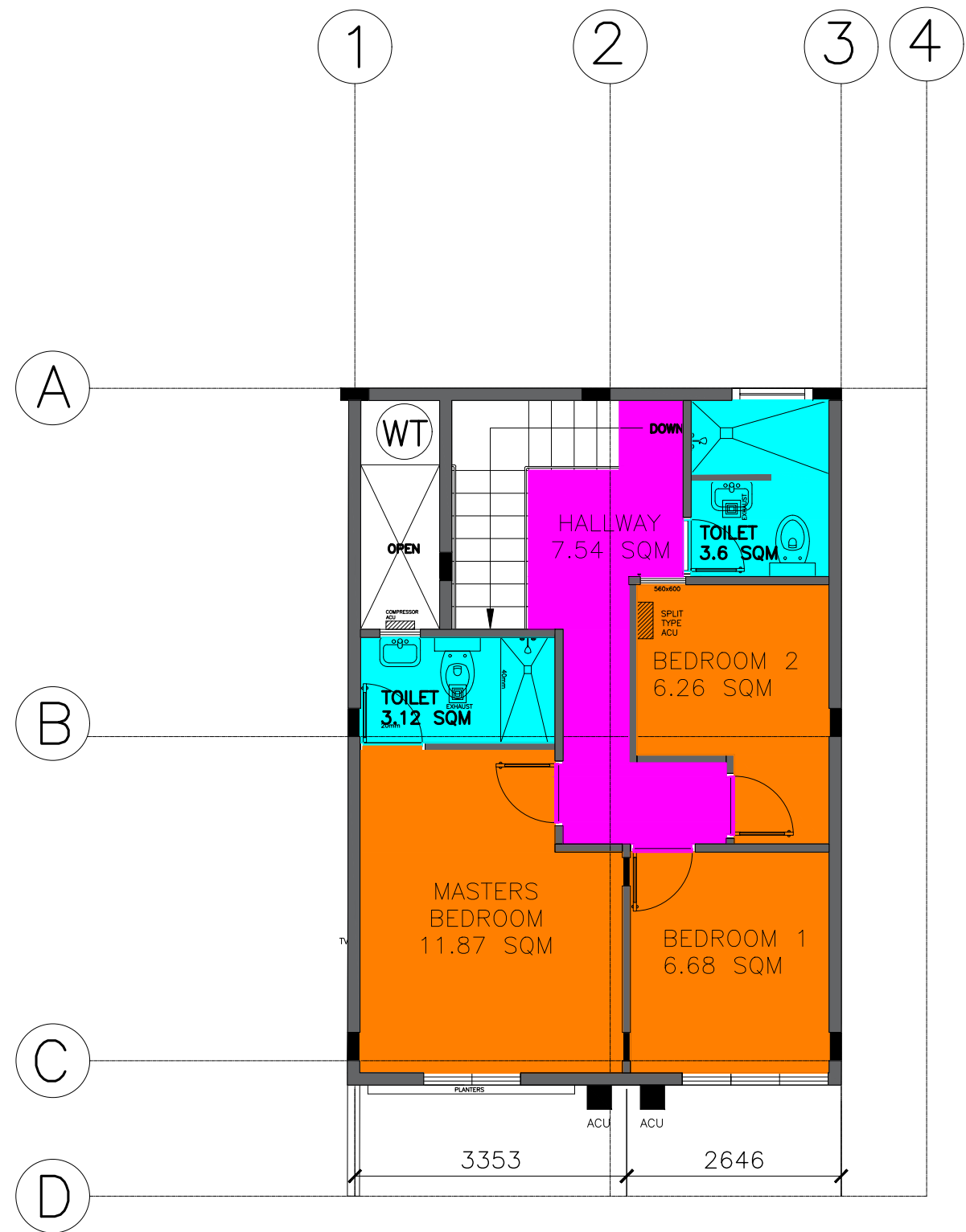
SECOND FLOOR PLAN HOREB
