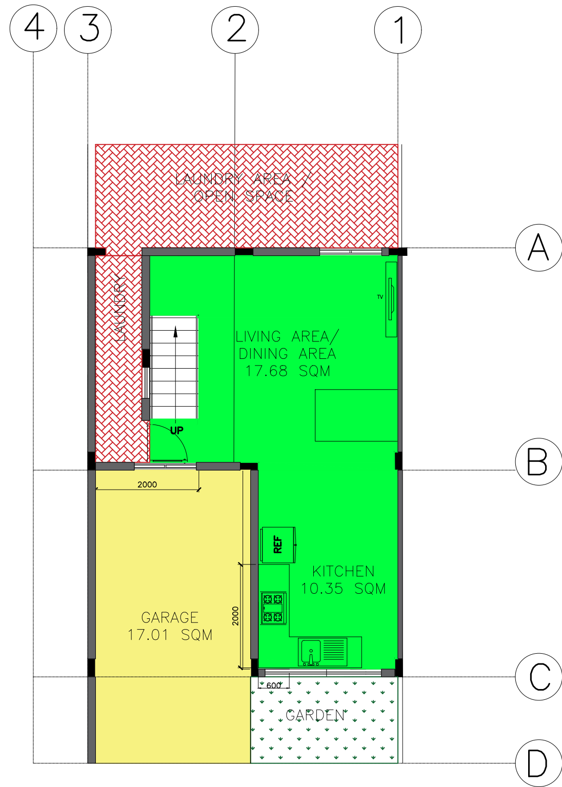
GROUND FLOOR PLAN HOREB
